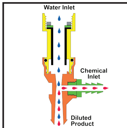
E-Gap technology mixes water with product while conforming to ASSE 1055B approved backflow prevention.
